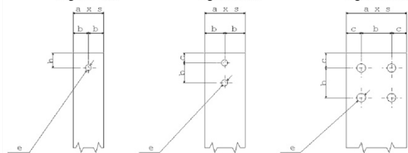
Terminali BT - Вводы HH - Terminals LV Fig.1 - Puc.1 Fig.2 - Puc.2 Fig.3 - Puc. 3
